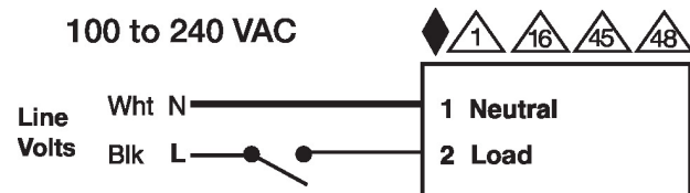
NEMA 4 Heater Option
