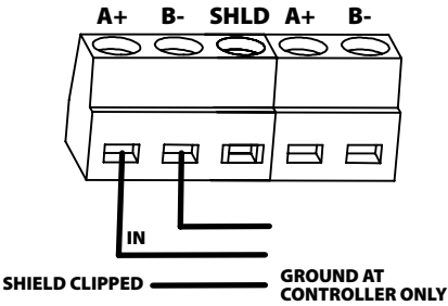
FIGURE 5: DAISY CHAIN WIRING
